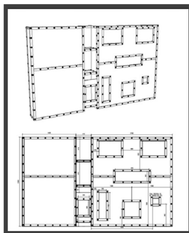
CAD Drawing
